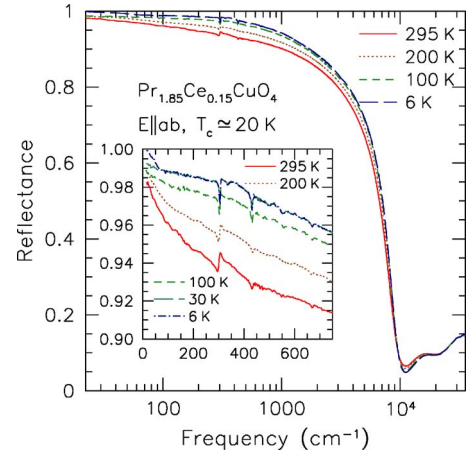
FIG. 1. (Color online) The temperature dependence of the reflectance at a near-normal angle of incidence of single crystal \text{Pr}_{1.85}\text{Ce}_{0.15}\text{CuO}_4 ( T_c \approx 20 \text{ K} ) from \approx 18 to 34\,000 \text{ cm}^{-1} for light polarized in the a - b plane above and below T_c . Inset: The detailed temperature dependence of the far-infrared reflectance above and below T_c . Note the kink and the sudden increase in the reflectance below \approx 70 \text{ cm}^{-1} for T \leq T_c . The sharp features in the reflectance are infrared-active lattice modes. (The resolution is 2 \text{ cm}^{-1} .)
