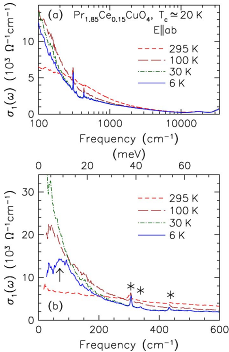
FIG. 2. (Color online) (a) The temperature dependence of the real part of the optical conductivity over a wide frequency range for \text{Pr}_{1.85}\text{Ce}_{0.15}\text{CuO}_4 above and below T_c for light polarized in the a - b planes. (b) The low-frequency optical conductivity. The conductivity in the normal state is described by a Drude component that narrows rapidly with decreasing temperature. Below T_c , there is a significant loss of spectral weight at low frequency (arrow) due to the formation of a condensate. The sharp features superimposed upon the electronic background at \approx 306 , 338 , and 433 \text{cm}^{-1} (asterisks) are infrared-active phonon modes (Ref. 43).
