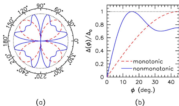
FIG. 6. (Color online) (a) A radial plot of the amplitude of an isotropic s -wave gap (dotted line), a monotonic d -wave gap, \Delta(\phi) = \Delta_0 \cos(2\phi) (dashed line), and a nonmonotonic d -wave gap, \Delta(\phi) = \Delta_0 [\cos(2\phi) - 0.42 \cos(6\phi) + 0.17 \cos(10\phi)] . Note that the gap functions are rotated by 45° with respect to the hole-doped cuprates. (b) A linear plot of the same gap functions over the first quadrant.
